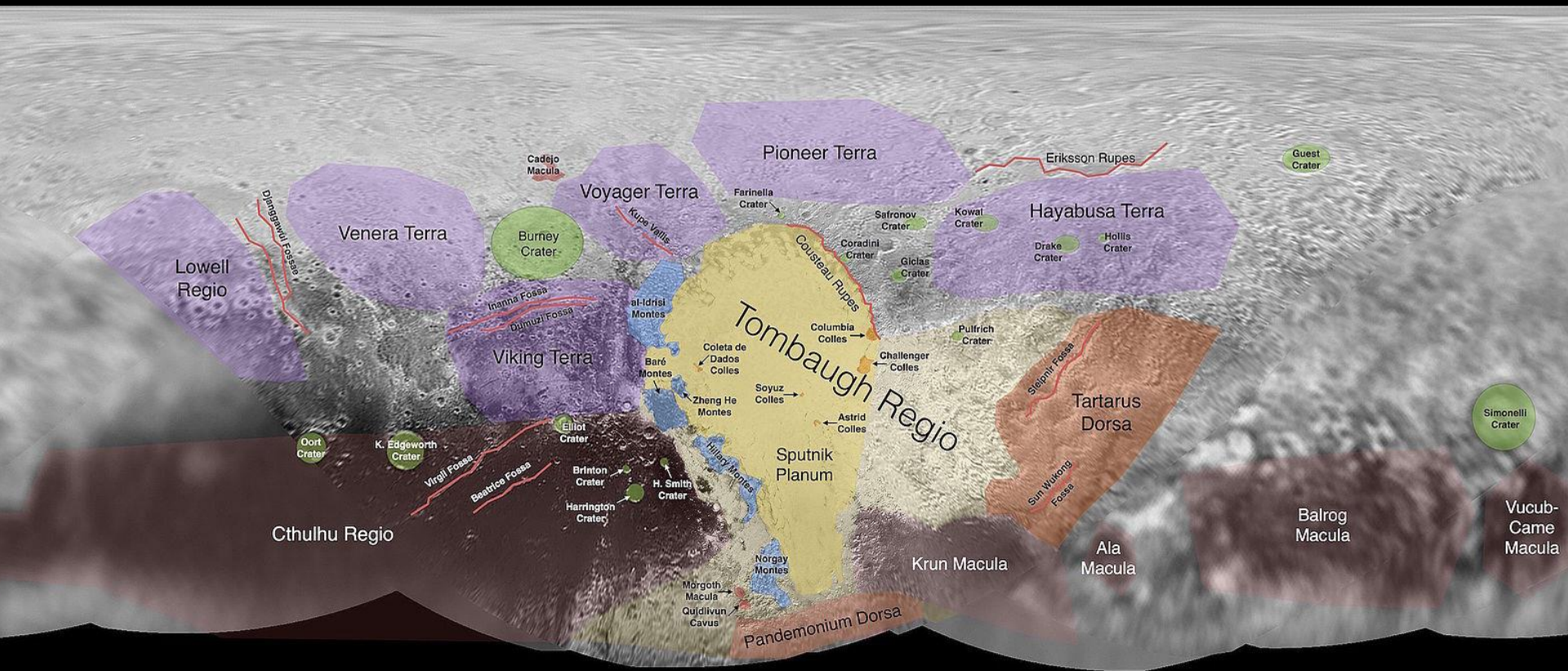
Informal Names for Features on Pluto
